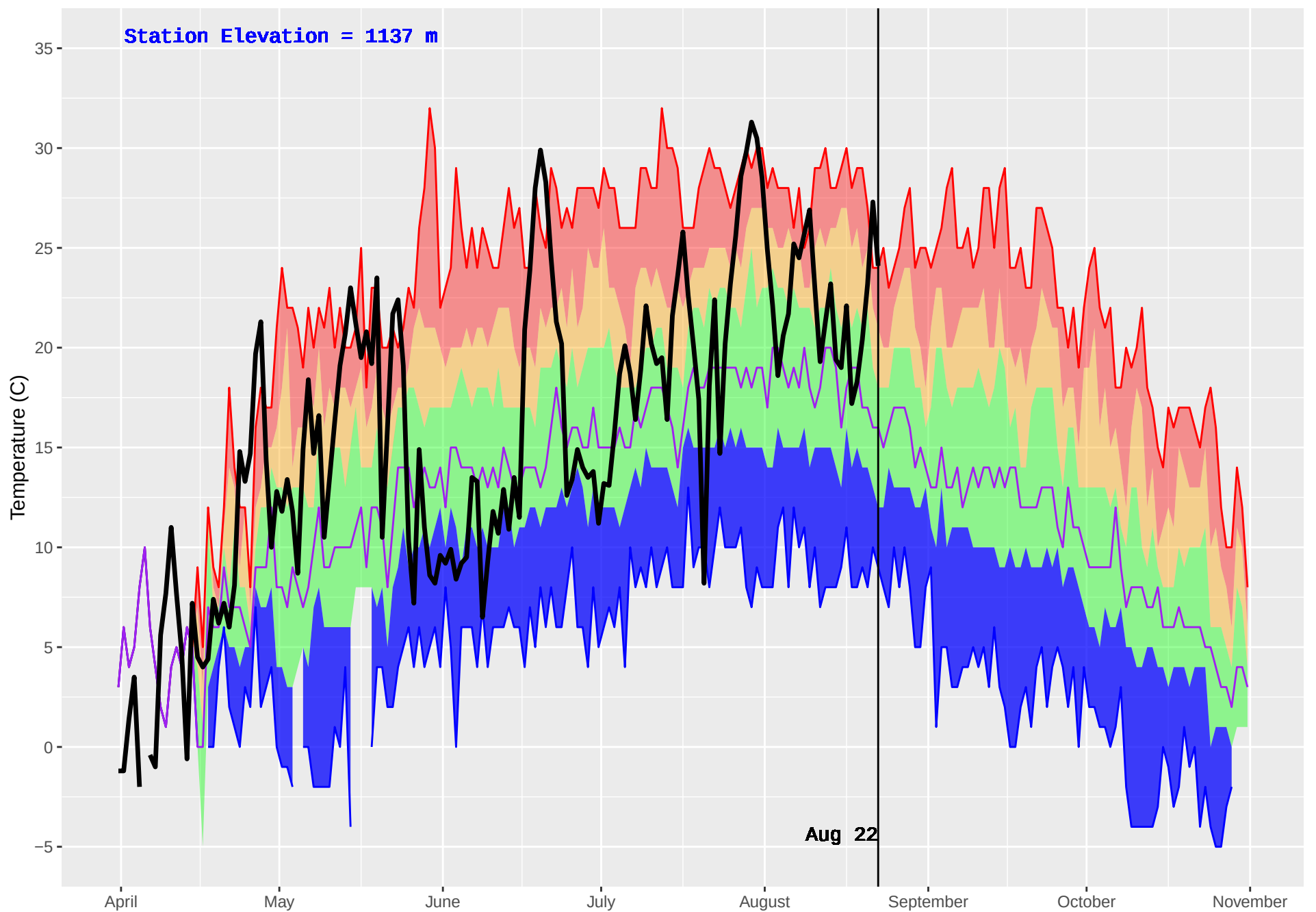
KLUSKUS (166) : Historical (1982–2016) and Current (2018) Daily Temperature
