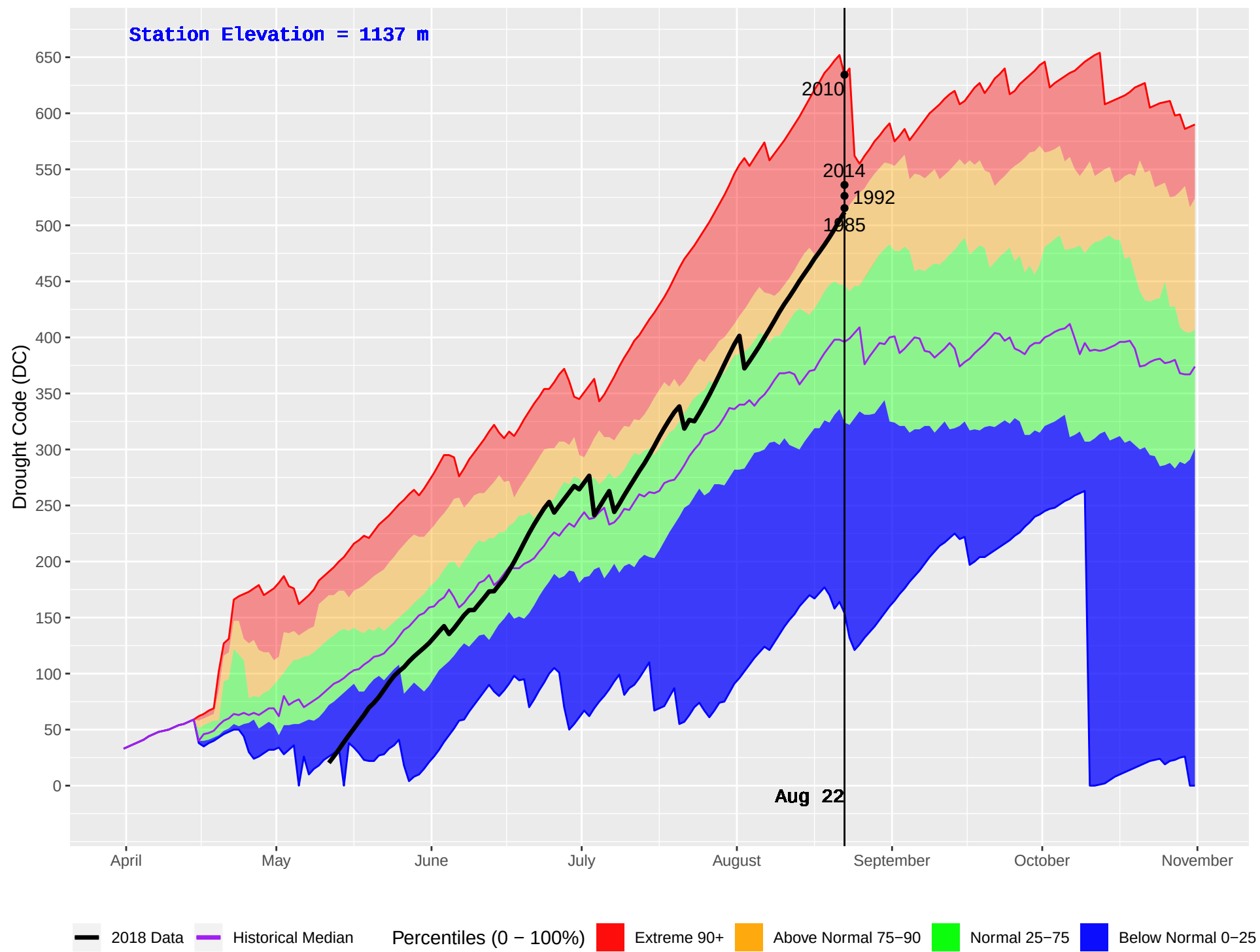
KLUSKUS (166) : Historical (1982–2016) and Current (2018) Daily Drought Code (DC)
