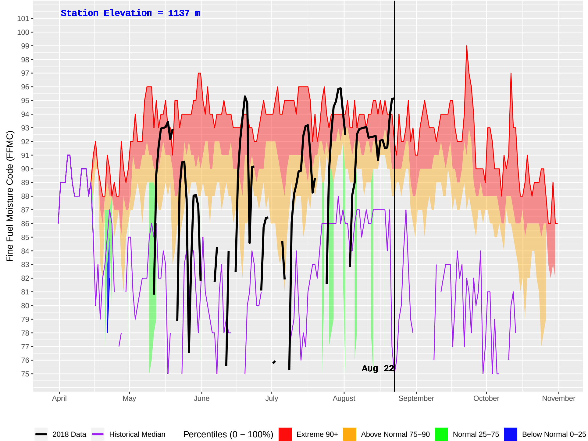
KLUSKUS (166) : Historical (1982–2016) and Current (2018) Daily Fine Fuel Moisture Code (FFMC)
