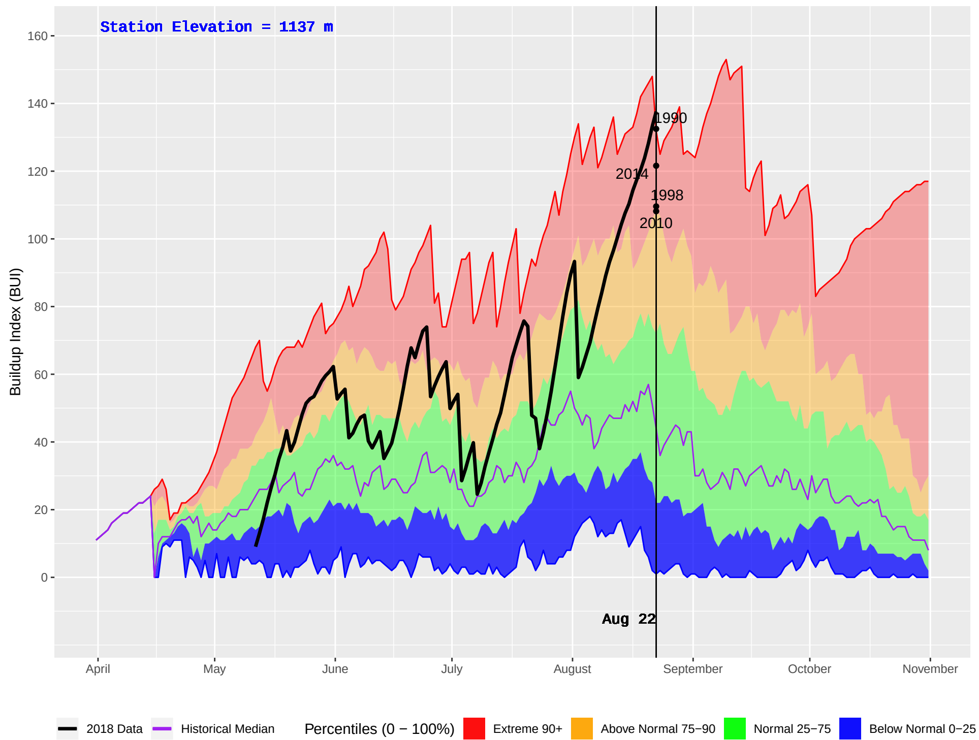
KLUSKUS (166) : Historical (1982–2016) and Current (2018) Daily Buildup Index (BUI)
