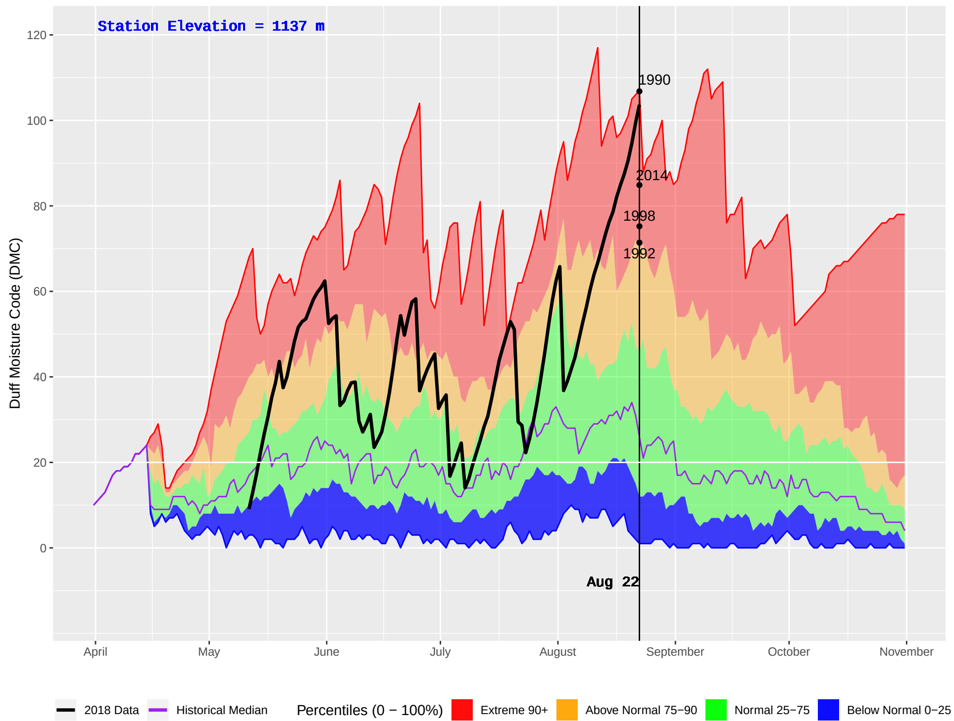
KLUSKUS (166) : Historical (1982–2016) and Current (2018) Daily Duff Moisture Code (DMC)
