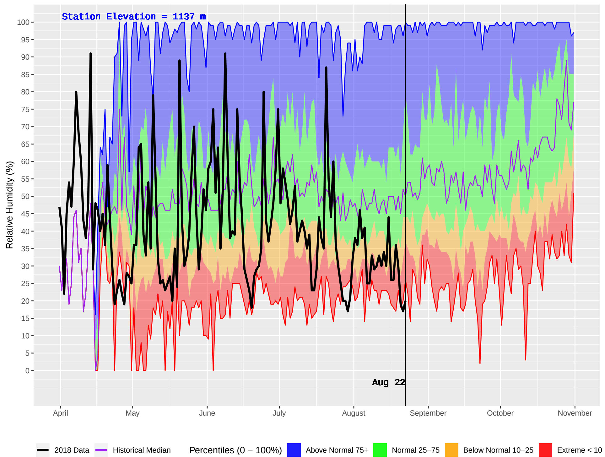
KLUSKUS (166) : Historical (1982–2016) and Current (2018) Daily Relative Humidity
