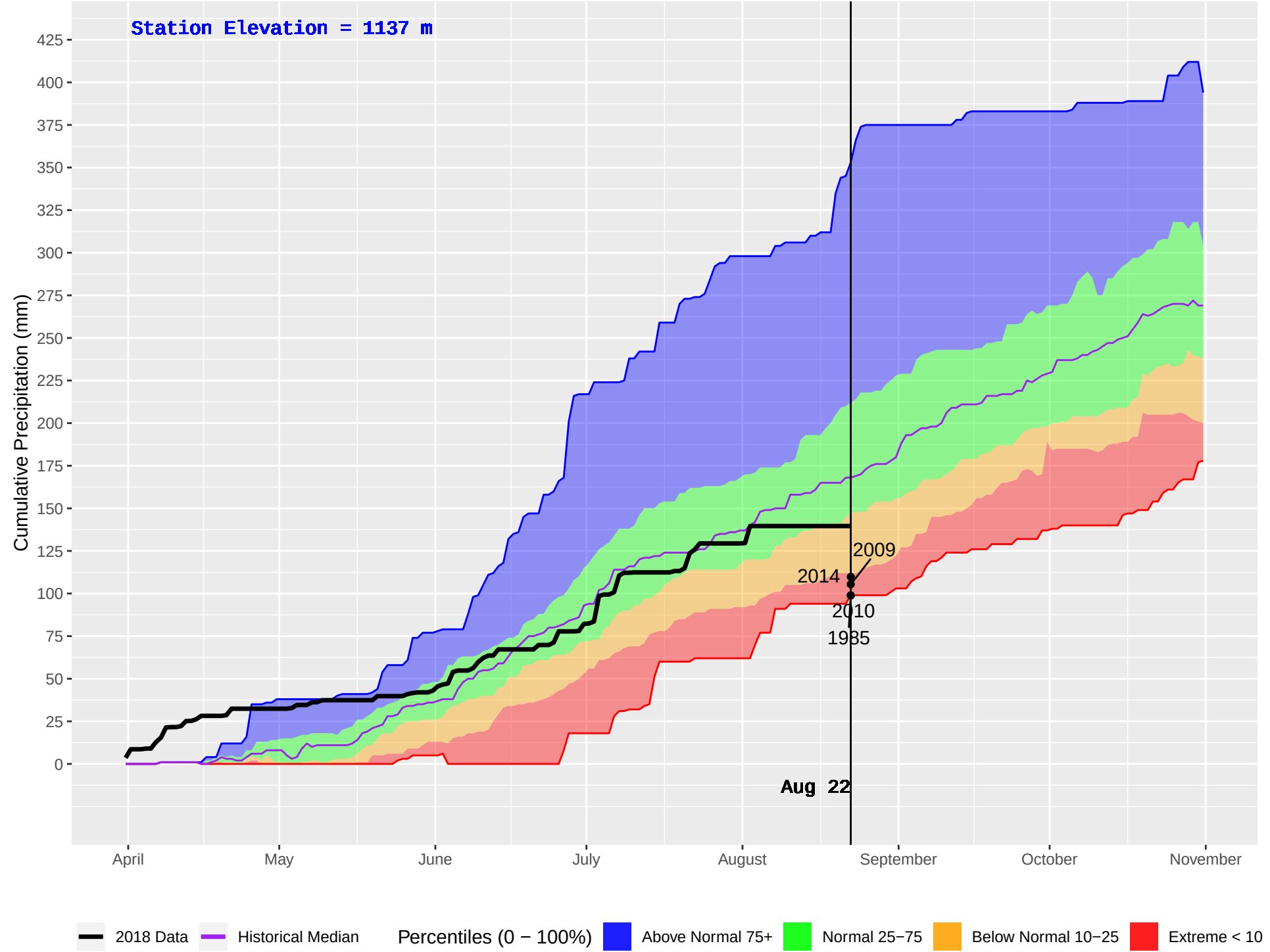
KLUSKUS (166) : Historical (1982–2016) and Current (2018) Daily Cumulative Precipitation
